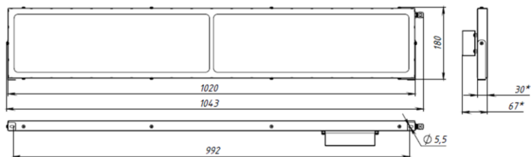
Titan Inox Standart 1000x180.
